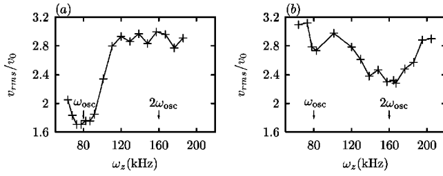
FIG. 6. rms width of the vertical velocity distribution obtained after 30 ms of cooling as a function of the Zeeman splitting between adjacent Zeeman levels. v_0 = \sqrt{\hbar m \omega_{\text{osc}}/2} is the rms width of the vibrational ground state. The polarization of the MB is linear in (a) and elliptical in (b).
